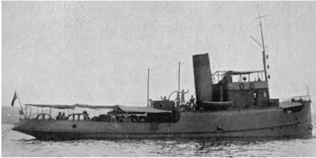
ATLANTE. 1936 ATLANTE (1928), ERCOLE (1928), AUSONIA (1920). 355 tons. Guns: 1—3 inch. H.P.: 900 = 11 kts.
